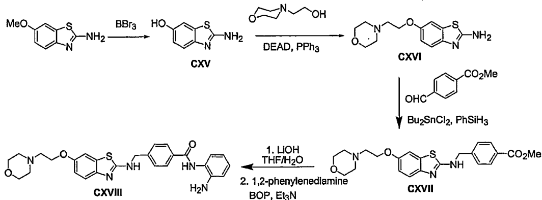
Scheme 33
